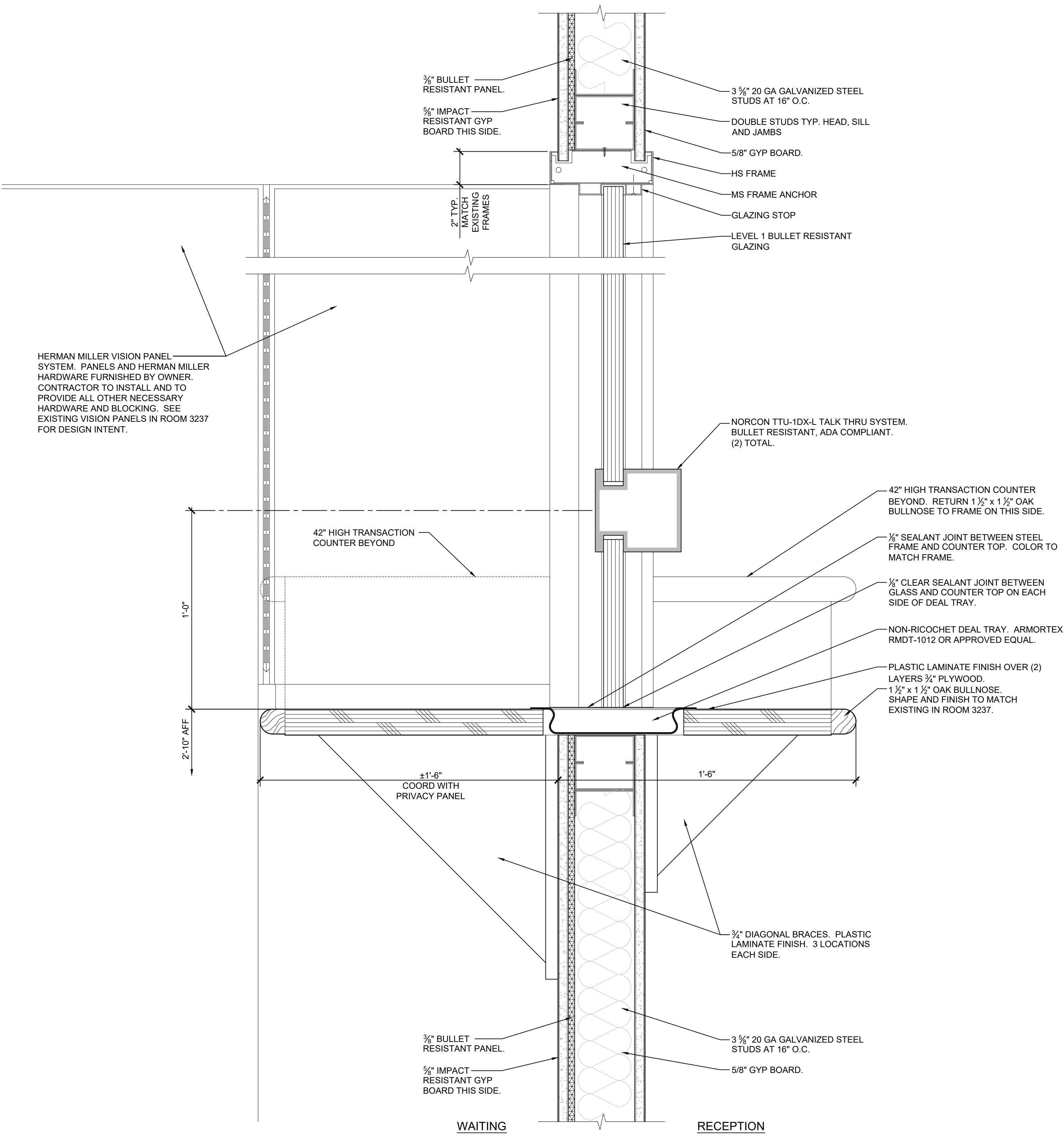
2 WINDOW SECTION scale 3"=1'-0"
