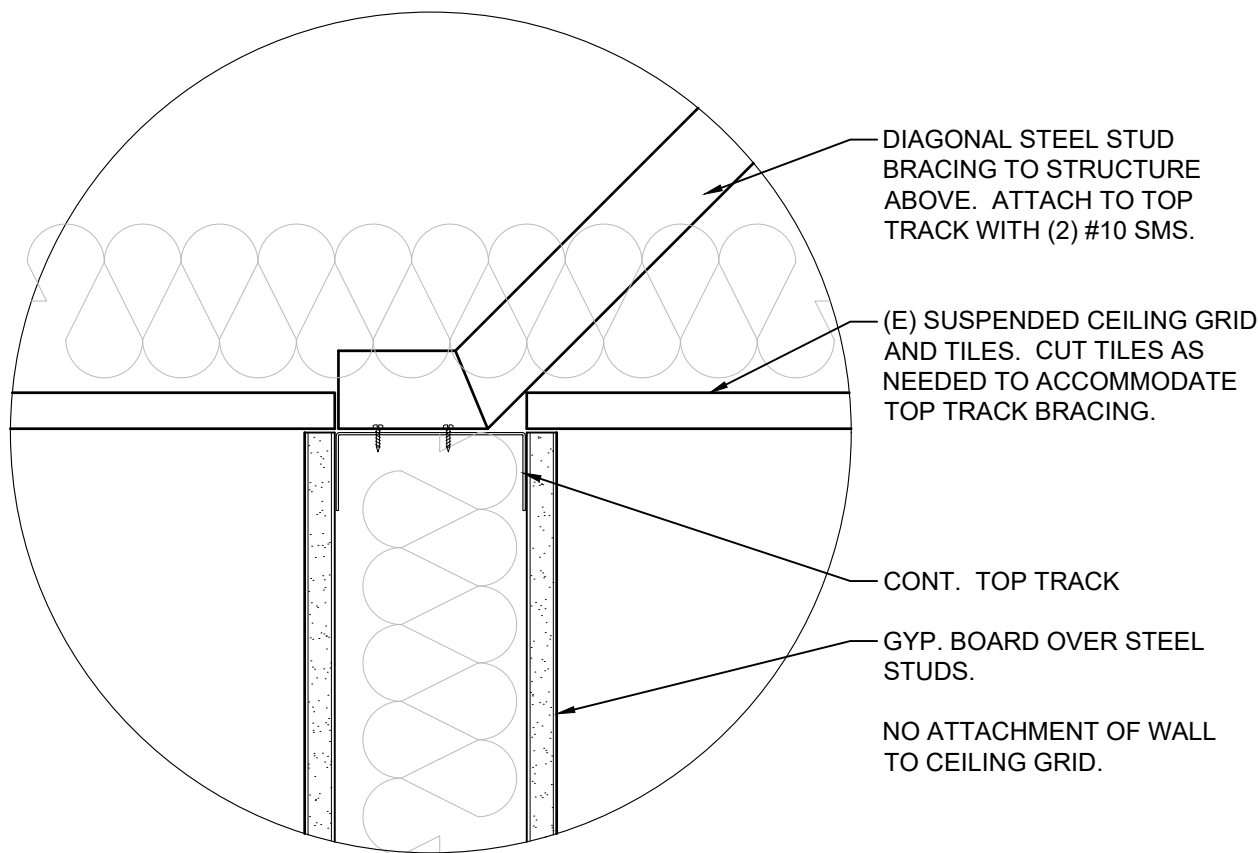
8 TOP OF WALL DETAIL scale 3"=1'-0"
