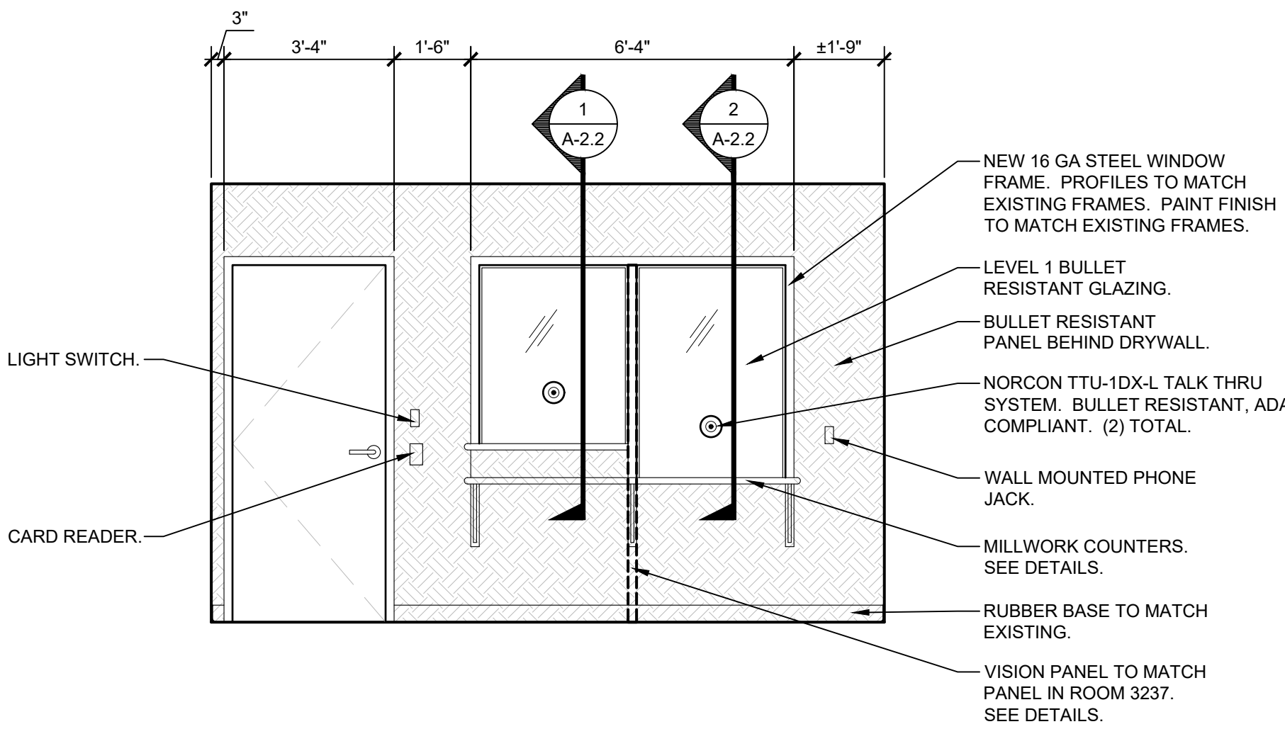
1 WAITING 3232 SOUTH ELEVATION scale 3/8"=1'-0"
