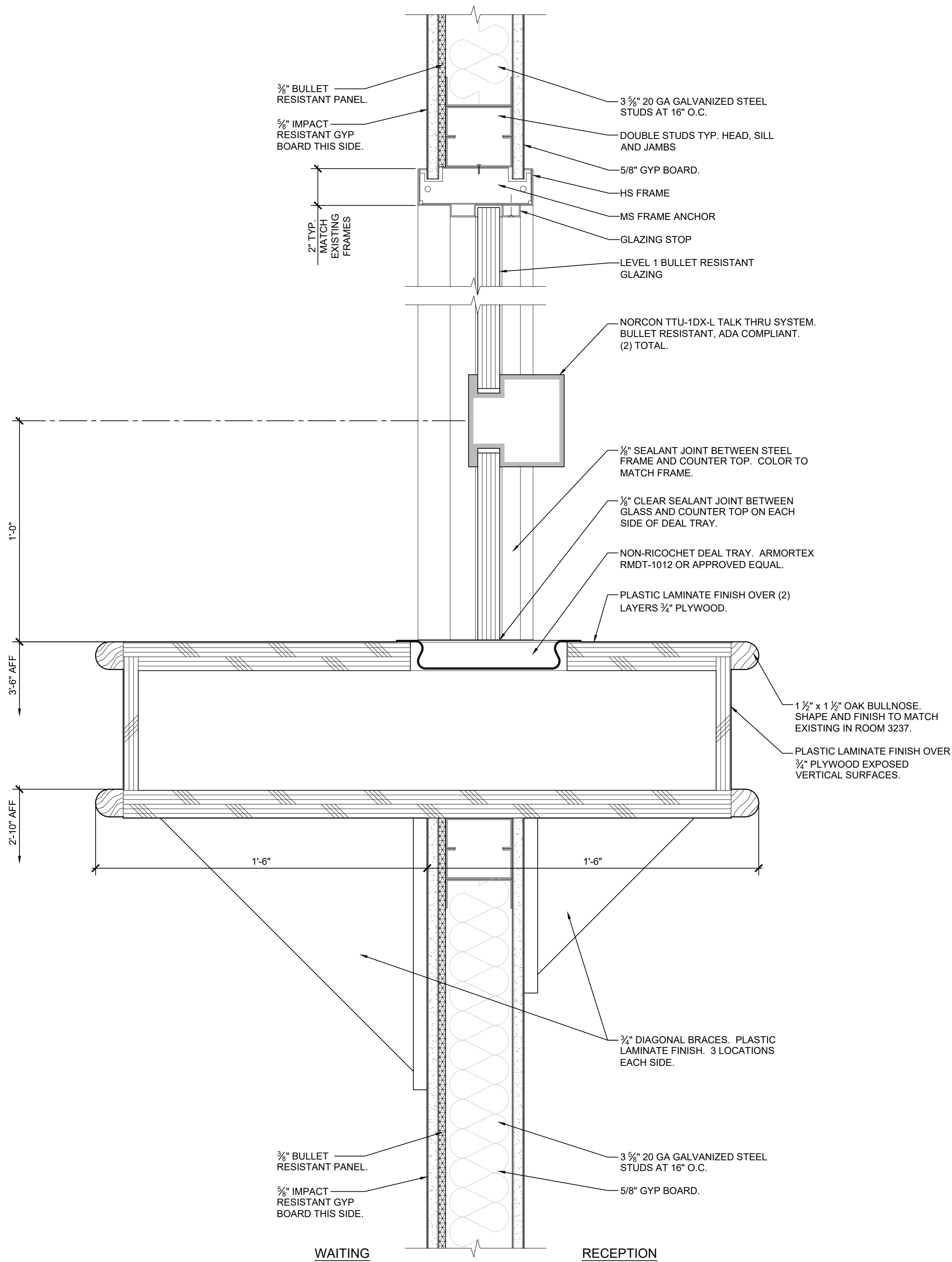
1 WINDOW SECTION scale 3"=1'-0"
