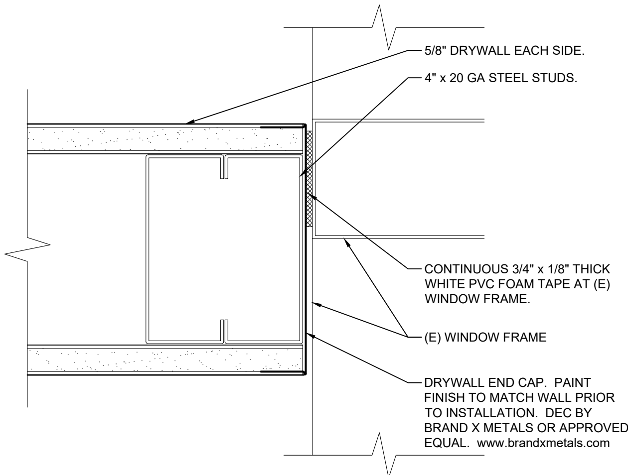
6 WALL PLAN DETAIL scale 6"=1'-0"
