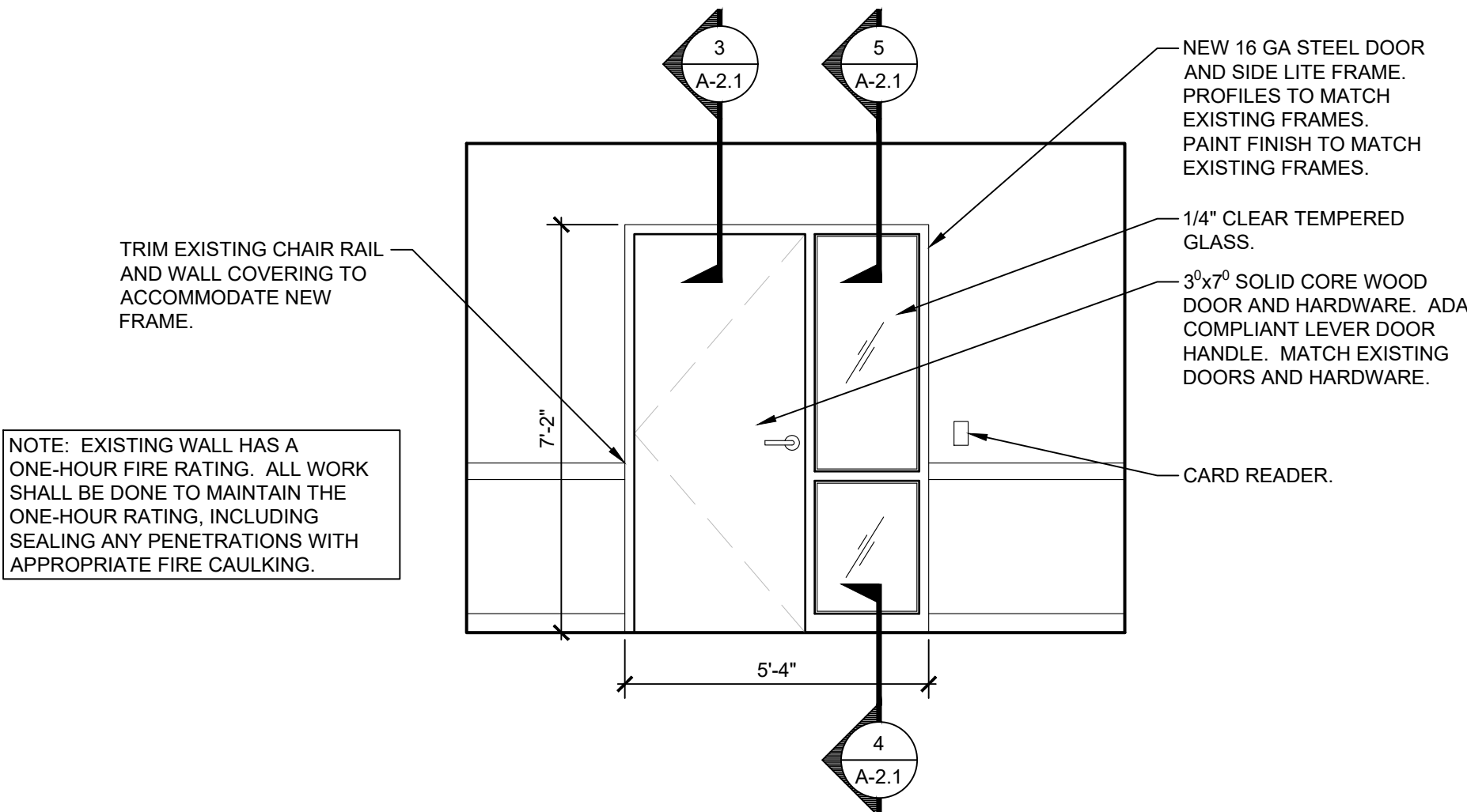
2 DOOR 3232A ELEV. (FROM CORR. 3241) scale 3/8"=1'-0"
