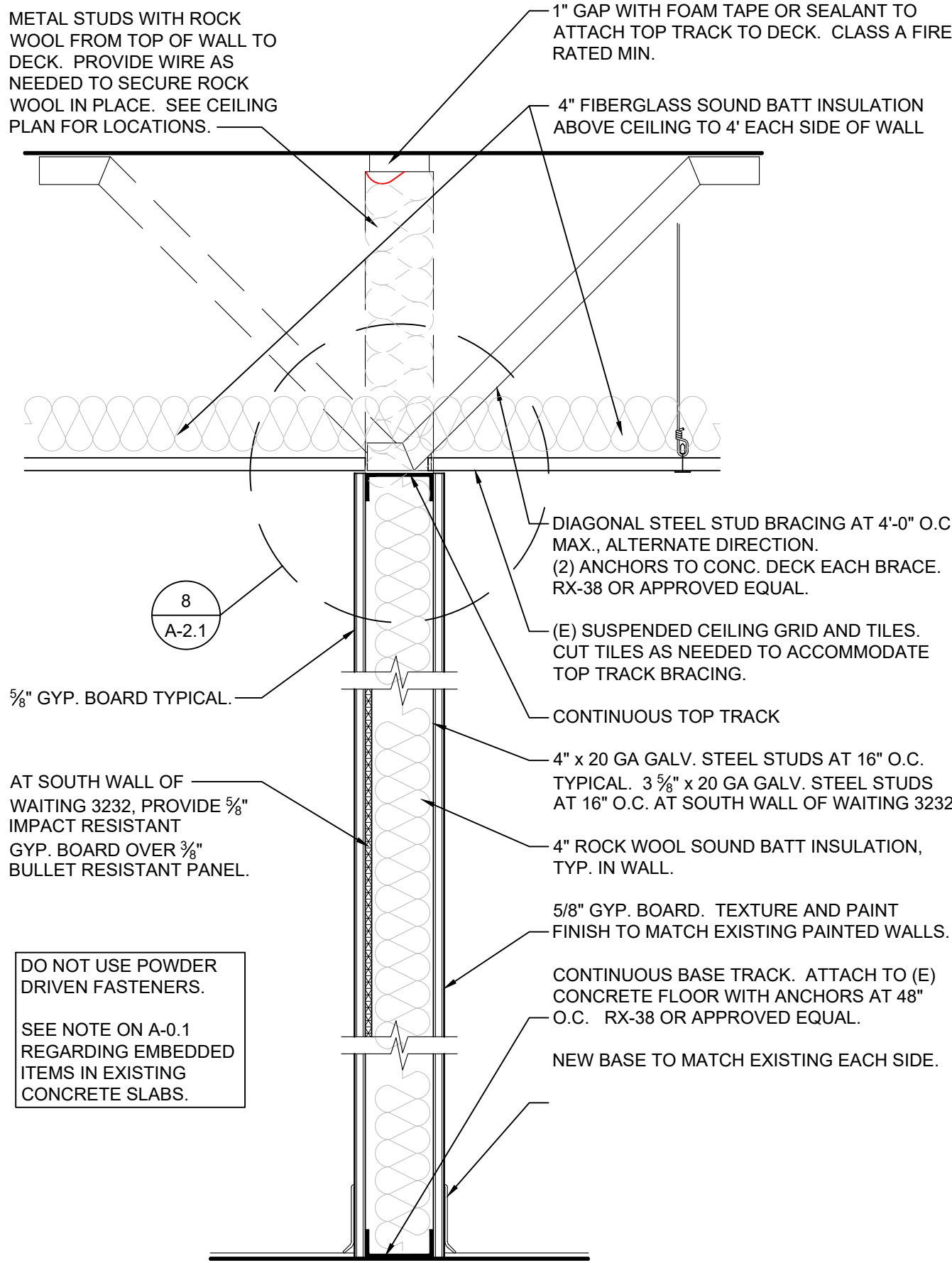
7 WALL SECTION scale 1 1/2"=1'-0"
