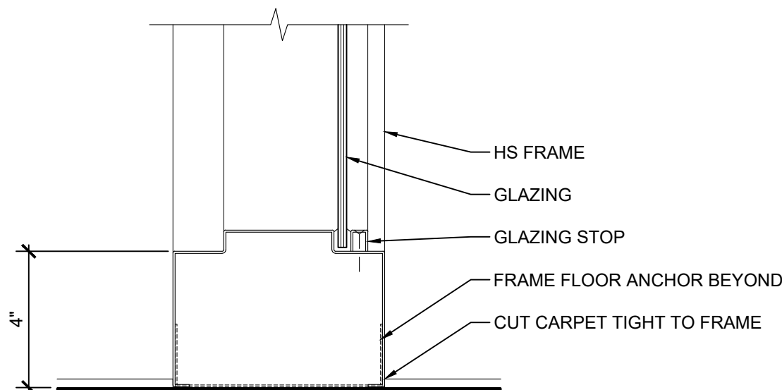
4 WINDOW SECTION scale 3"=1'-0"
