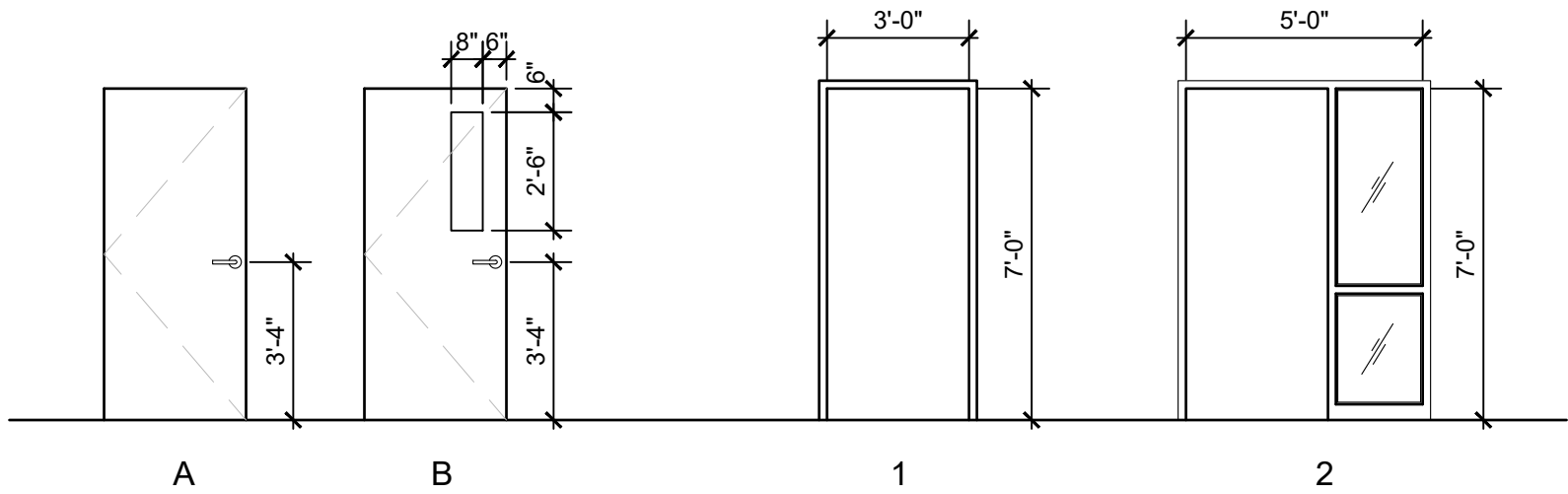
DOOR AND FRAME TYPES scale 1/4" = 1'-0"
