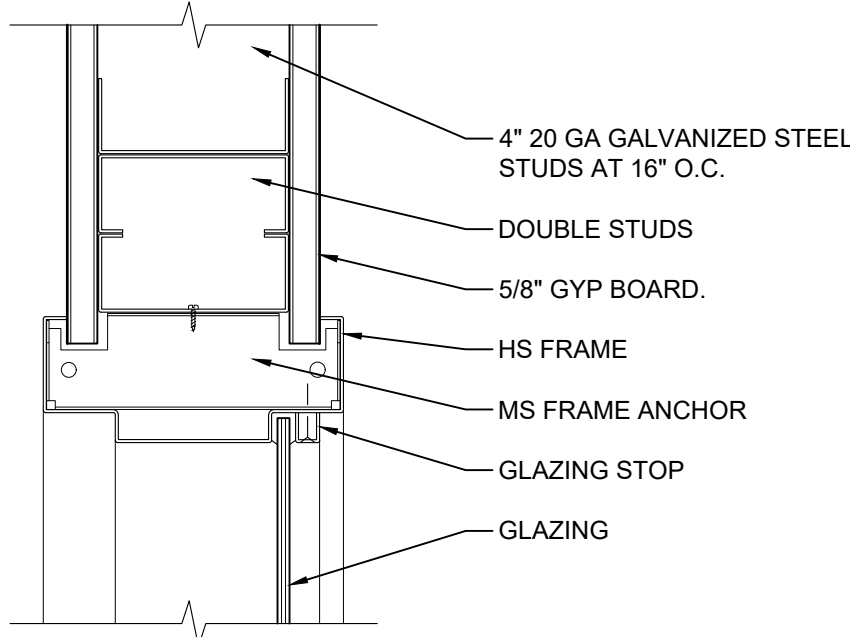
5 WINDOW HEAD (JAMB SIM) scale 3"=1'-0"
